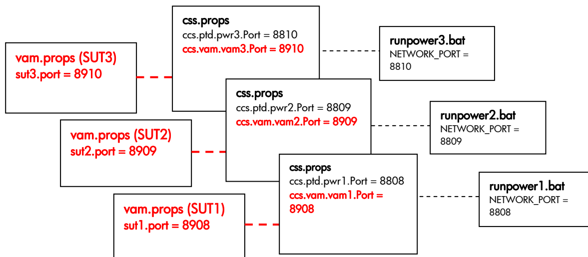
Figure 7.3 – Describes TCP port coordination with multiple SUTs
